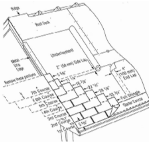
Typical roof-covering material example.
